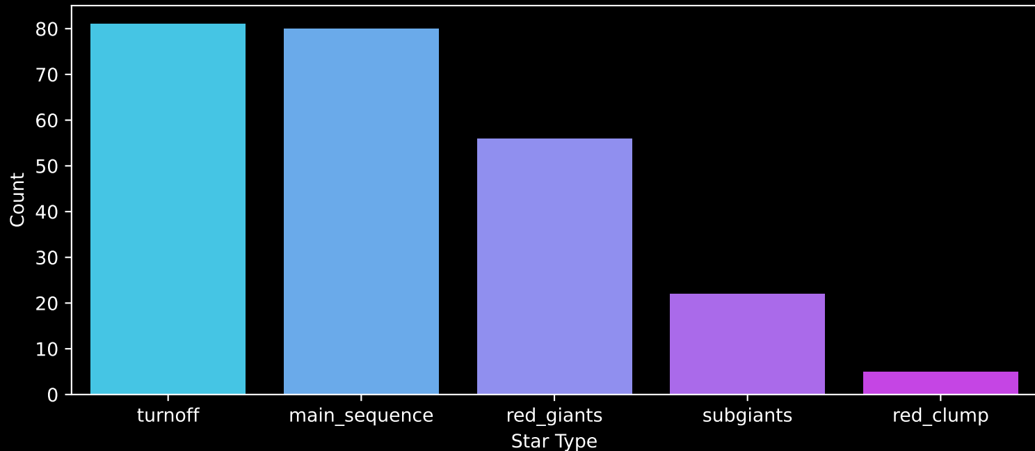
GALAH DR4 Field: [7149] Count plot of Star Type
