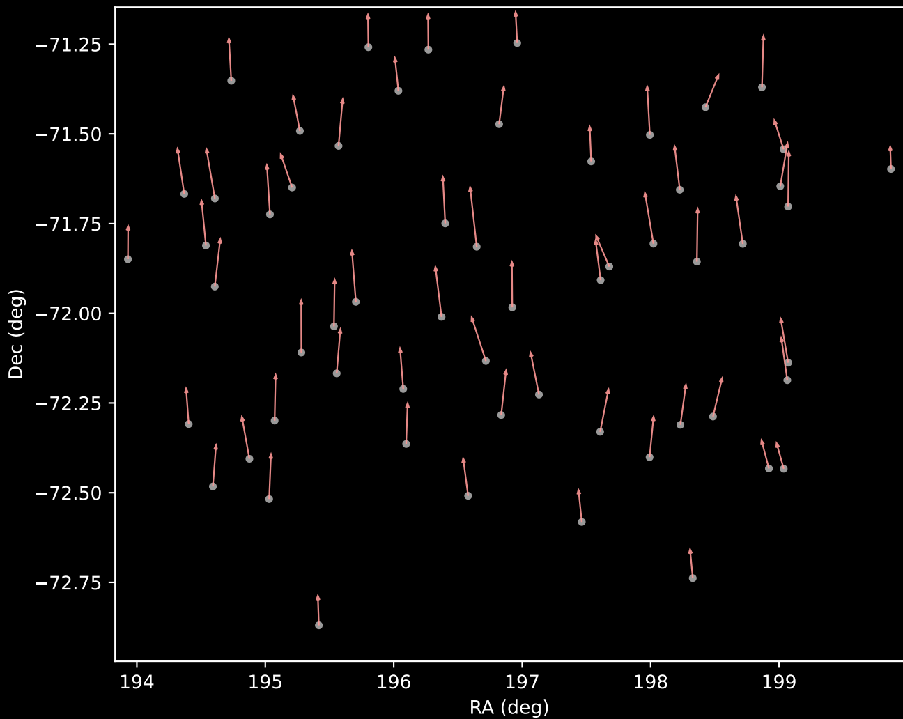
GALAH DR4 Cluster 7 Proper Motion Vectors (n=59)
