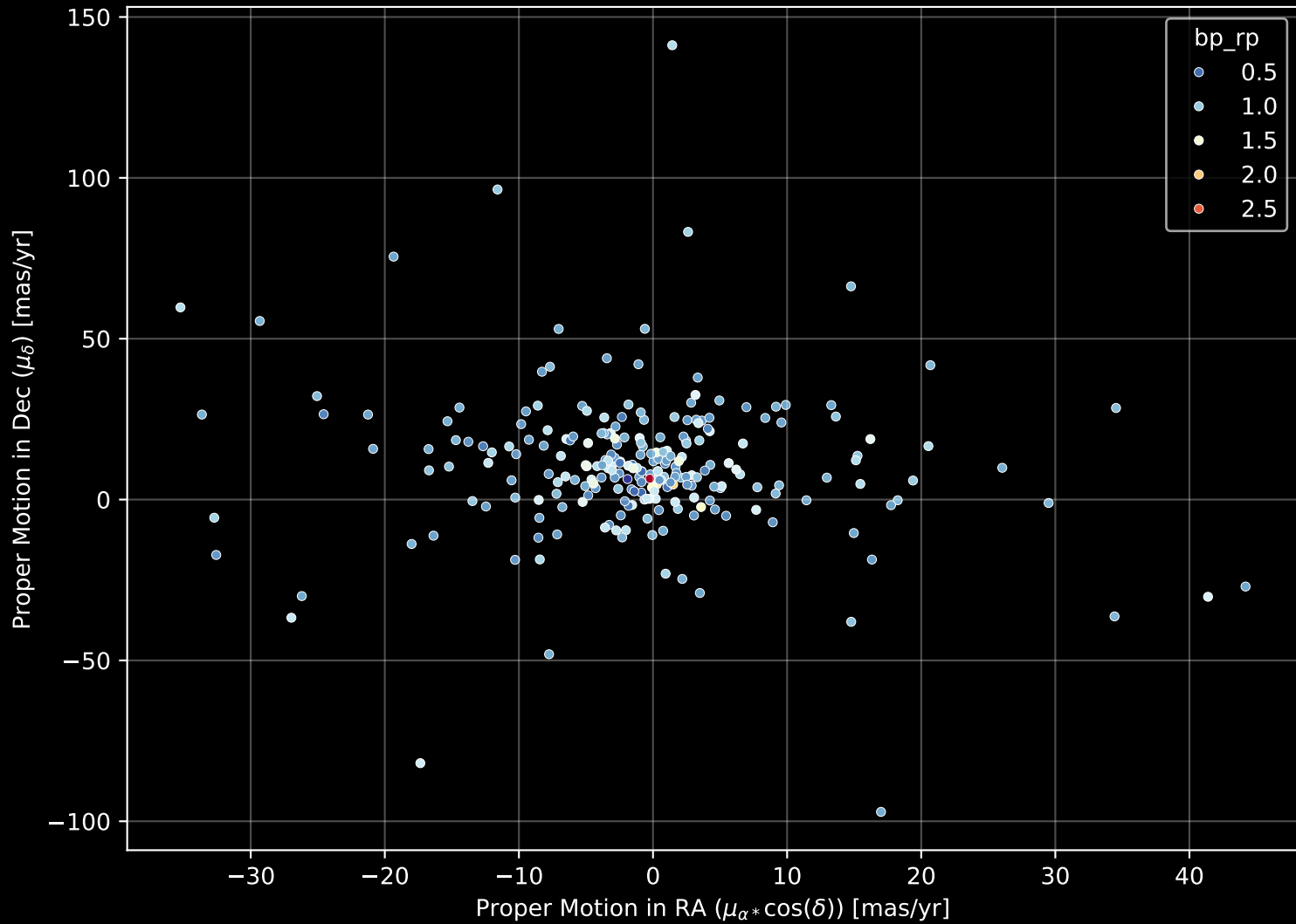
GALAH DR4 Field: [7149] Proper Motion Diagram (n= 244)
