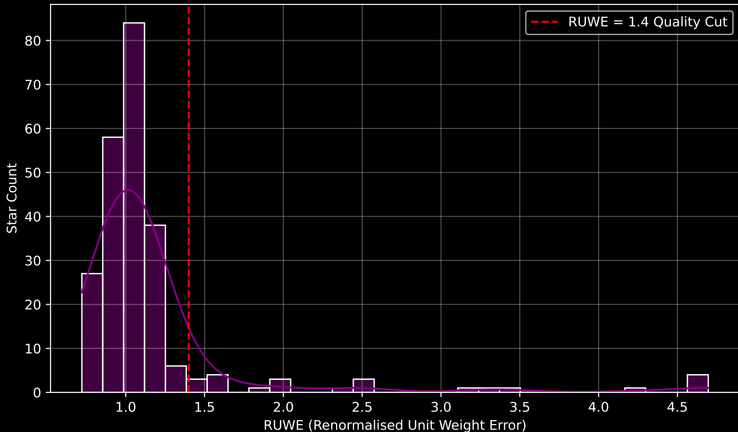
GALAH DR4 Field [7149] RUWE Distribution (n= 236)
